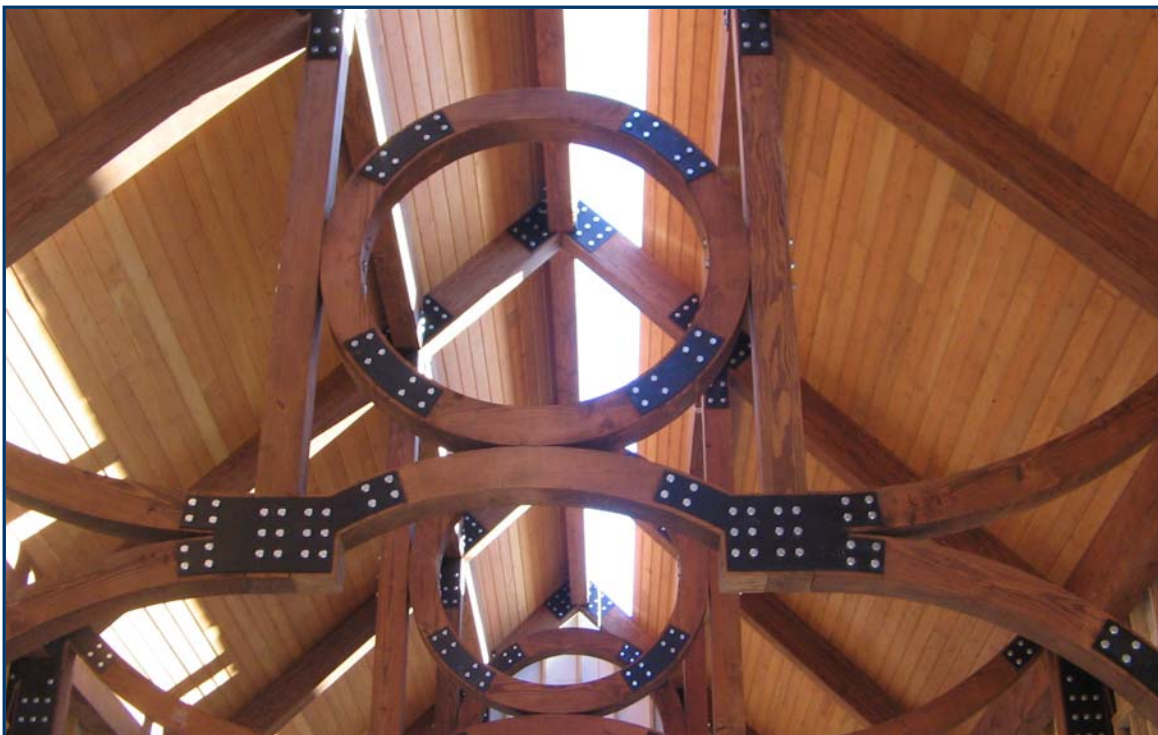
January 26, 2006 – View of Ceiling and Timber Framing from inside Riverfront Station
